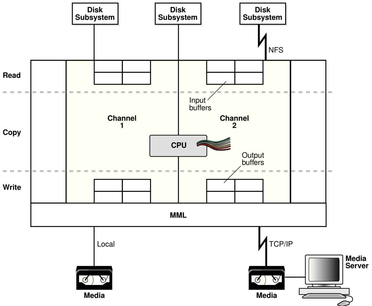
Figure 23-2 Phases of a Multichannel Backup to Tape
