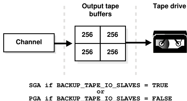
Figure 23-4 Allocation of Tape Buffers
